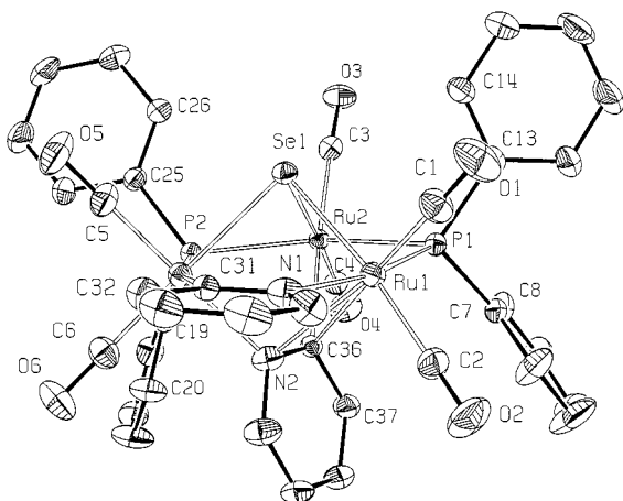
Figure 1. ORTEP diagram (30% probability level) of the molecular structure of 1 showing the atom numbering scheme; selected interatomic distances (Å): Ru(1)–Se(1) 2.515(1), Ru(1)–P(1) 2.433(1), Ru(1)–N(1) 2.173(2), Ru(1)–N(2) 2.619(3), Ru(1)–C(36) 2.822(3), Ru(2)–Se(1) 2.599(1), Ru(2)–P(1) 2.395(1), Ru(2)–P(2) 2.404(1), Ru(2)–C(36) 2.147(2), Ru(3)–Se(1) 2.550(1), Ru(3)–P(2) 2.416(1), Ru(3)–N(2) 2.171(2), Ru(3)–C(31) 2.128(2), N(1)–C(31) 1.348(3), N(2)–C(36) 1.353(3), Ru(1)···Ru(2) 3.351(1), Ru(1)···Ru(3) 3.442(1), Ru(2)···Ru(3) 3.476(1).
